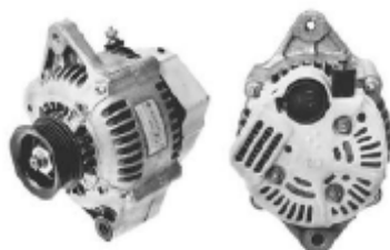
13879 102211-2351 12V/80A
