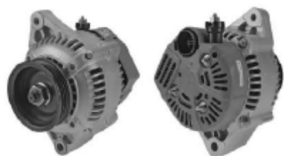
13508 100211-3690 12V/55A
