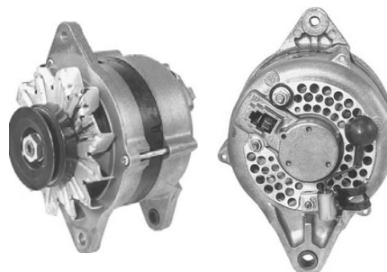
14131 12V/45A 021000/0530/0590/1350 /1820/1850/1890/3220/3730 TOYOTA 1969-75
