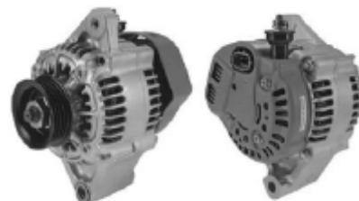
13409 100211-0200 12V/70A
