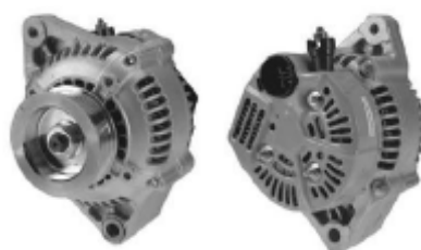
14759 100211-1350.100211-1351 12V/60A
