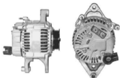
13836 102211-0690 12V/120A
