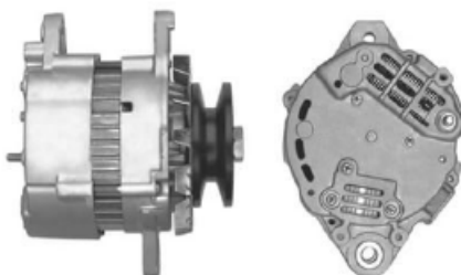
12V/110A 37000-4300A
