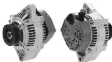
14679 100211-1180.100211-1050 12V/60A
