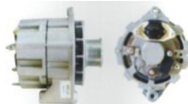
BXF1259A 12V/85A 0120484042
