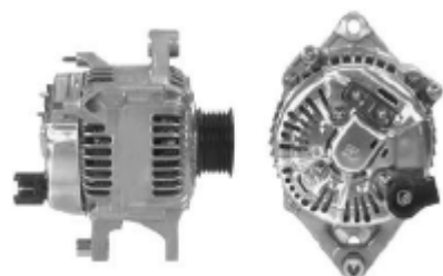
13763 121000-4231 12V/120A
