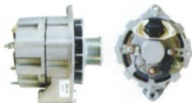
AL114 24V/45A 9120080114
