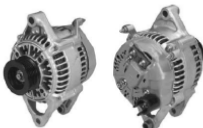
13185 121000-3360.121000-2660 12V/75A
