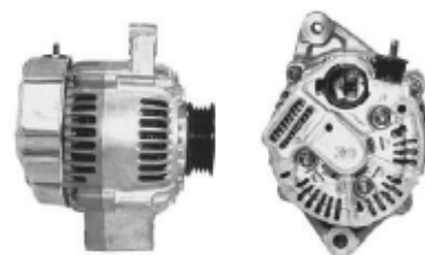
13397 100211-7470.100211-9780 12V/70A
