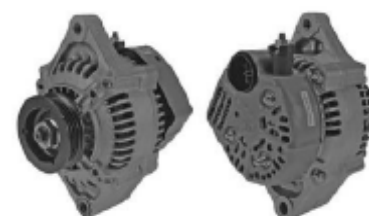
14755 100211-2210.100211-2211 12V/60A
