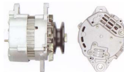
JA1789IR 12V/80A 37300-22650
