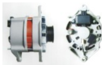
BXH1236A 12V/55A 0120488314
