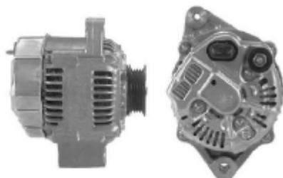
13457 101211-5970 12V/70A
