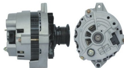
12V/85A CA1385IR 96224431
