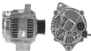
13453 121000-4130 12V/120A
