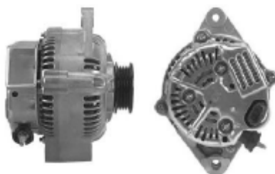
13536 101211-0350.101211-5090 12V/70A
