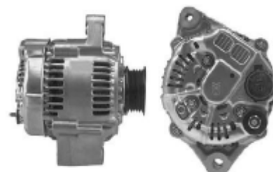
13339 100211-7180.100211-3430 12V/60A
