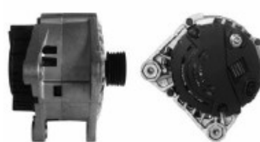
CA1778IR 12V/150A 0986049161
