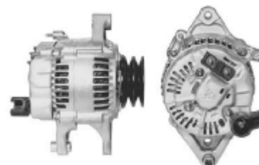
13956 101211-7440 12V/100A
