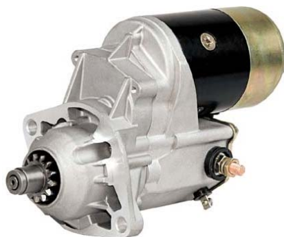
QD6225C 2-1526-ND 128000-021 128000-054 12V/2.5KW/13T CUMMINS
