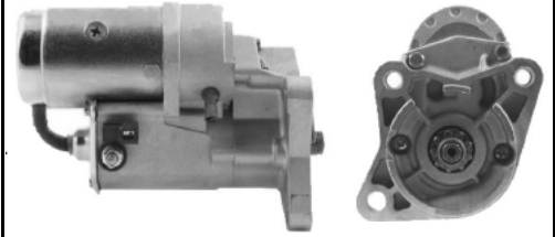
QDJ1208A-000 31354 12V/20. KW/9T/CW
