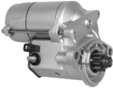
2-2732-ND 18139 12V/2.0KW/11T/CW 228000-2970
