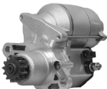
17263/17400 2-1404-ND 12V/1.4KW/13T/CCW 128000-7390
