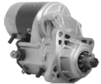
2-1037-ND 16830 12V/2.5KW/11T/CW 028000-5580 TOYOTA
