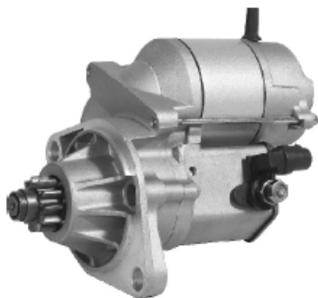
17788 2-1983-ND 12V/1.4KW/11T/CW 228000-7430
