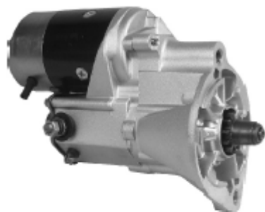
19748 24V/4.5KW/11T/CW 12V/2.5KW/11T/CW TOYOTA 13B 14B
