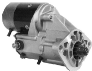
QDJ2206X16-000 24V/4.5KW/11T/CW
