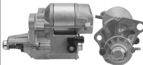
2-1981-ND 17785 12V/1.4KW/10T/CW 228000-7420
