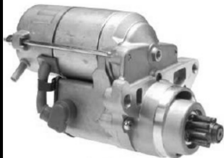
17665 12V/1.6KW/9T/CW 228000-5040
