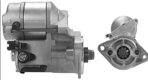
2-2060-ND 17793 12V/1.2KW/9T/CW 228000-7740
