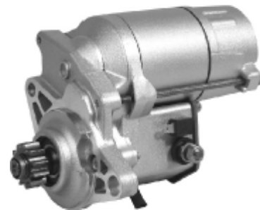
12V/1.7KW/11T/CCW 228000-4960
