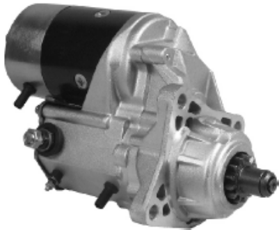
QDJ1206B-000 QDJ1206B-000 17548 2-1739-ND 12V/2.7KW/13T/CW
