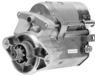
2-1459-ND 17216 12V/1.4KW/11T/CW
