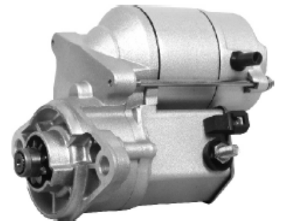
16737 2-1034-ND 12V/1.0KW/9T/CW 028000-5900
