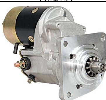
QD6225C 2-1526-ND 128000-021 128000-054 12V/2.5KW/13T CUMMINS
