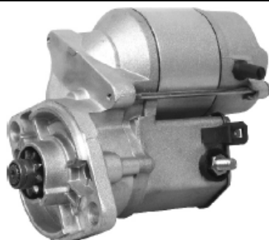
16828 2-1040-ND 12V/1.0KW/9T/CW 028000-8220
