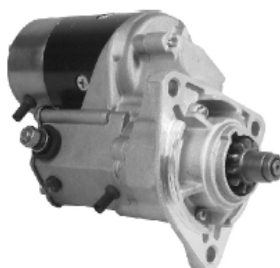
18190 2-2105-ND 24V/4.5KW/11T/CW 12V/4.5KW/11T/CW 028000-6200
