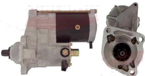
QDJ2273H-000 2-2234-ND 19516 24V/5.5KW/11T/CW 6SD1
