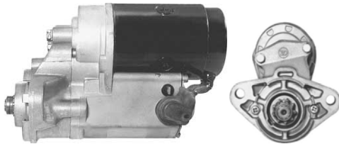
2-1044-ND 16826 12V/1.0KW/9T/CW 028000-8050 TOYOTA COROLLA
