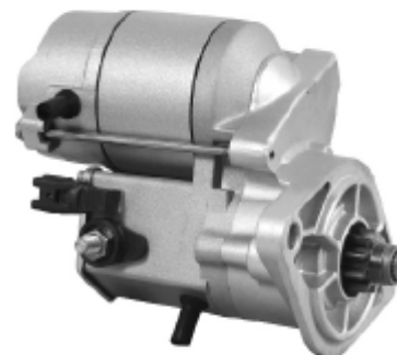
SND22A04 24V/1.4KW/9T/CW
