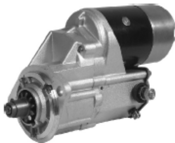
2-2708-ND 17290 12V/2.5KW/11T/CW 128000-4110
