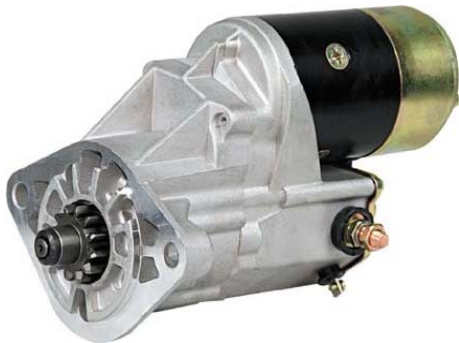
QD6232 28100-17030 24V/4.5KW/12T TOYOTA
