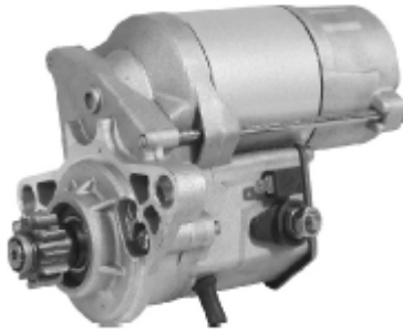
SND13A25 12V/2.0KW/11T/CCW
