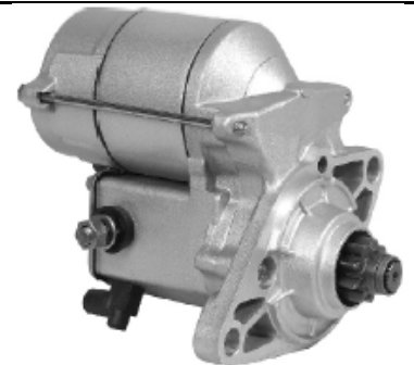
17517 2-1715-ND 12V/1.4KW/9T/CW 228000-2060
