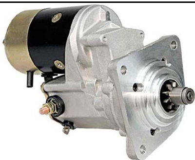
QD6222A 128000-1060 17380 12V/2.5KW/10T
