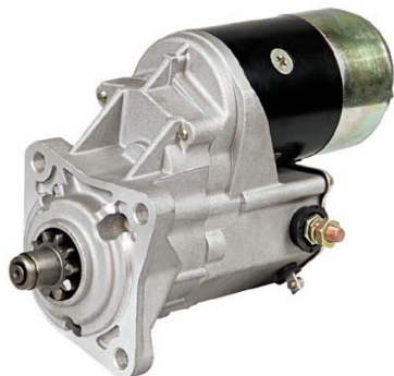
QD6222A 128000-1060 17380 12V/2.5KW/10T
