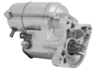
17084 2-1383-ND 12V/1.4KW/10T/CW 128000-4960
