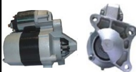
D7E19 12V/0.85KW/8T/CW
