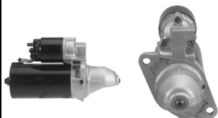
0001-109-040 12V/1.7KW/9T/CW
