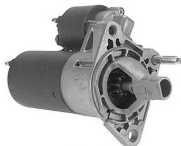
0001-108-134 12V/1.4KW/9T/CW
