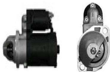
LESTER: 18951 0001-223-021 12V/2.2KW/9T/CW
