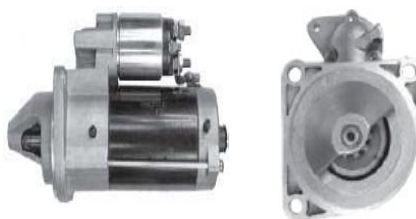
LESTER:18374 0001-230-007 12V/3.0KW/9T/CW
