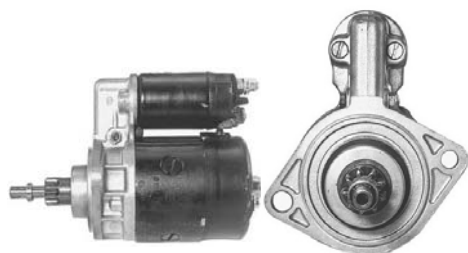
LESTER: 16974 0001-208-420 12V/9T/0.95KW/CW
