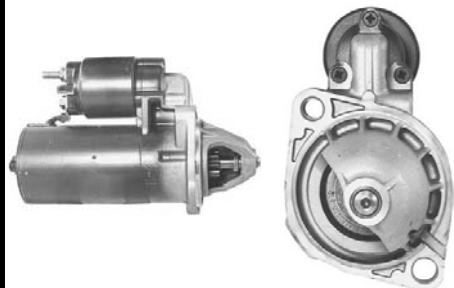
LESTER: 17276 0001-108-092 12V/1.4KW/9T/CW
