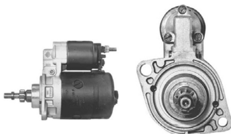
0001-211-253 12V/0.8KW/9T/CCW
