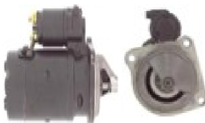
0001-368-020 24V/4.0KW/9T
