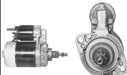
0001-208-428 12V/0.95KW/9T/CCW
